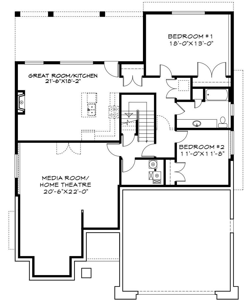
BASEMENT / FOUNDATION PLAN GROSS AREA = 1707 SQUARE FEET
