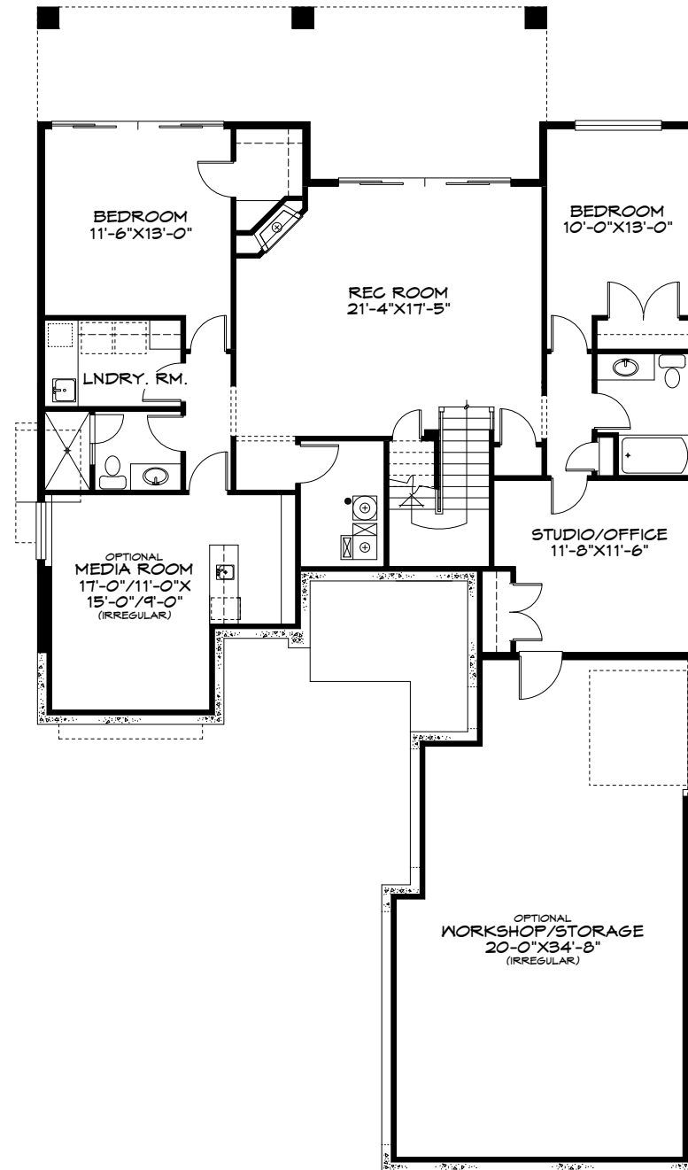
BASEMENT/FOUNDATION PLAN GROSS AREA = 2382 SQUARE FEET
