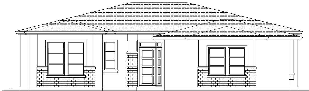
ELEVATION B FRONT ELEVATION WITHOUT ENTRY WING
