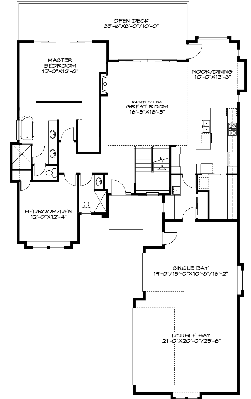
MAIN FLOOR PLAN FINISHED AREA = 1671 SQUARE FEET
