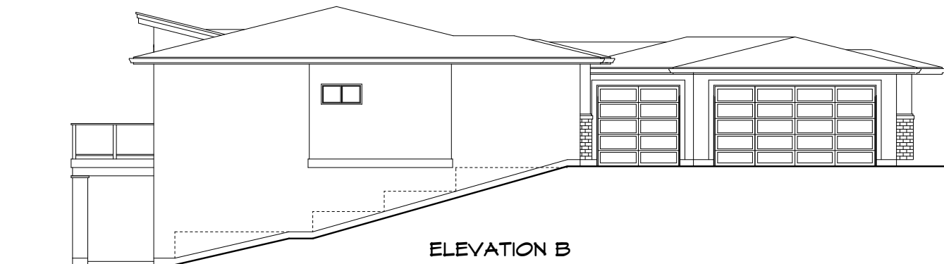
ELEVATION B FRONT ELEVATION WITHOUT ENTRY WING
