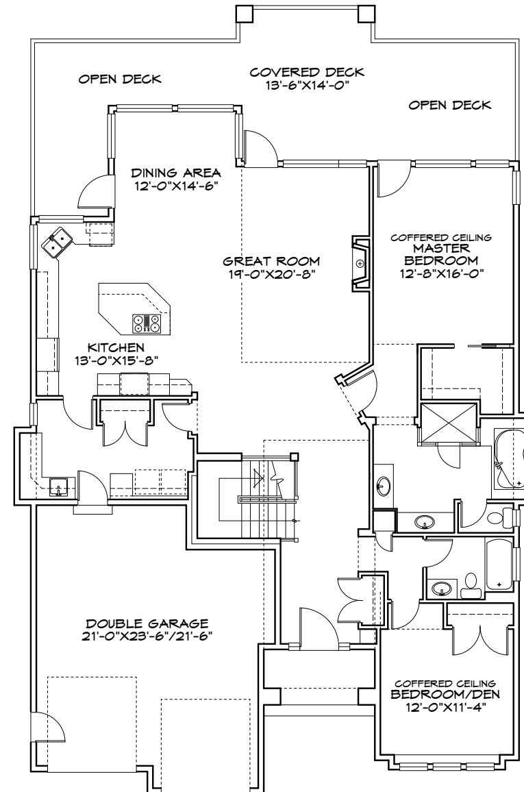
MAIN FLOOR PLAN FINISHED AREA = 1941 SQUARE FEET
