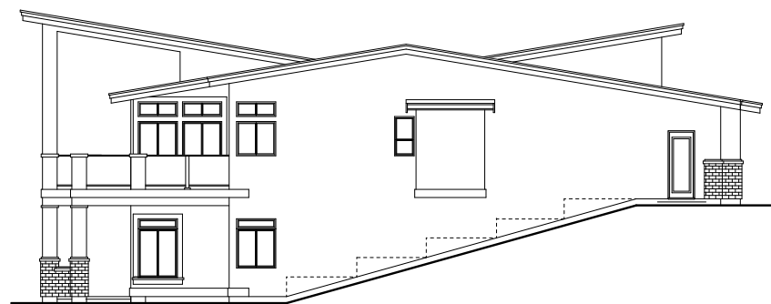
ELEVATION B SIDE ELEVATION WITHOUT ENTRY WING OR COVERED DECK
